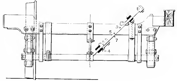
Fig. 1537. End Elevation.
